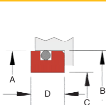
O-Ring Mounted
