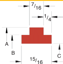
T-Shape Standard
