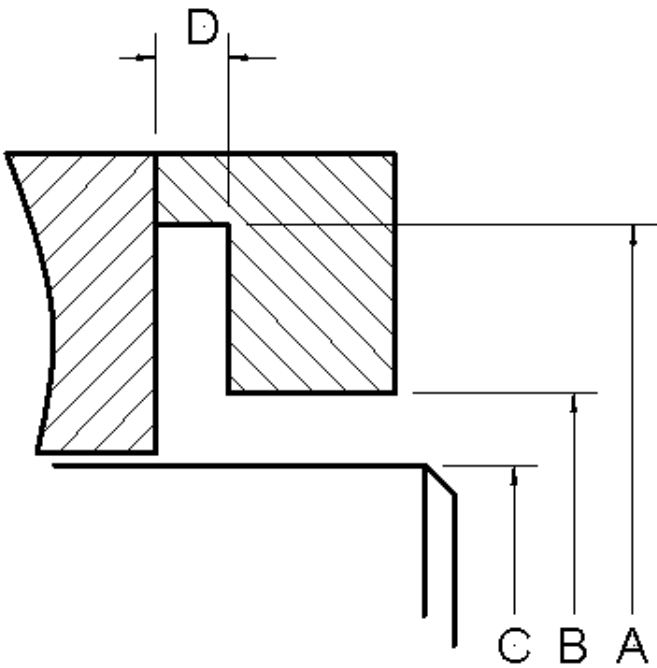
Hardware Dimensions
