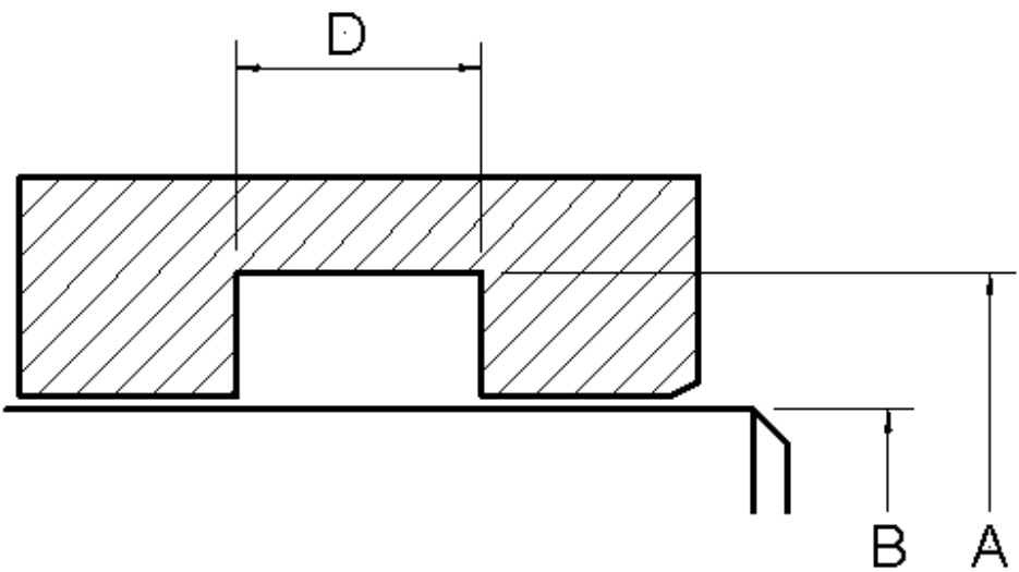
Hardware Dimensions
