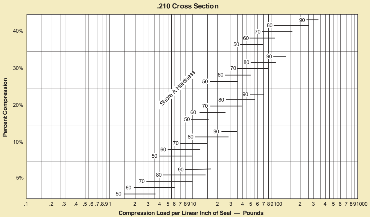
Figure 2-7: .210 Cross Section
