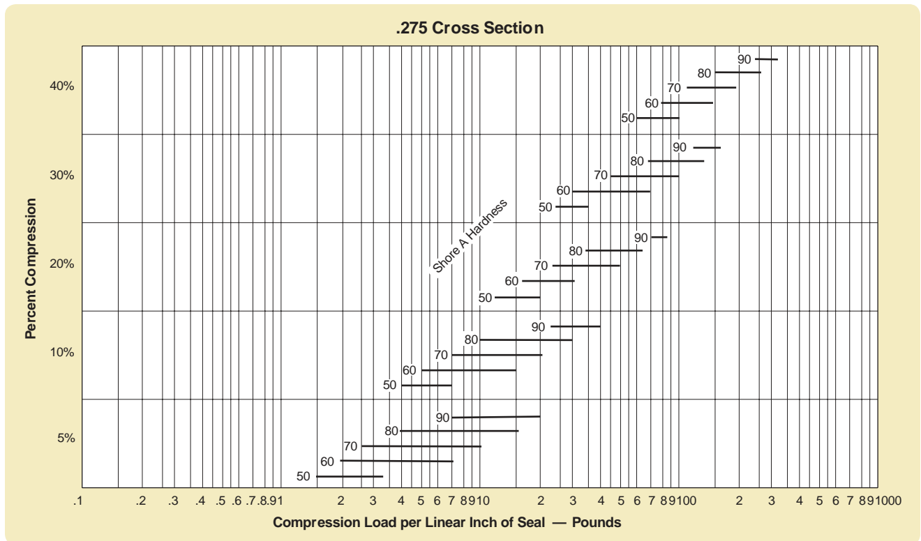
Figure 2-8: .275 Cross Section
