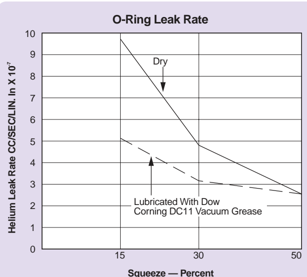
Figure 3-8: O-ring Leak Rate
