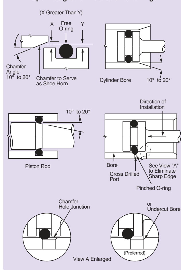
Figure 3-4: Proper Designs for Installation of O-rings
