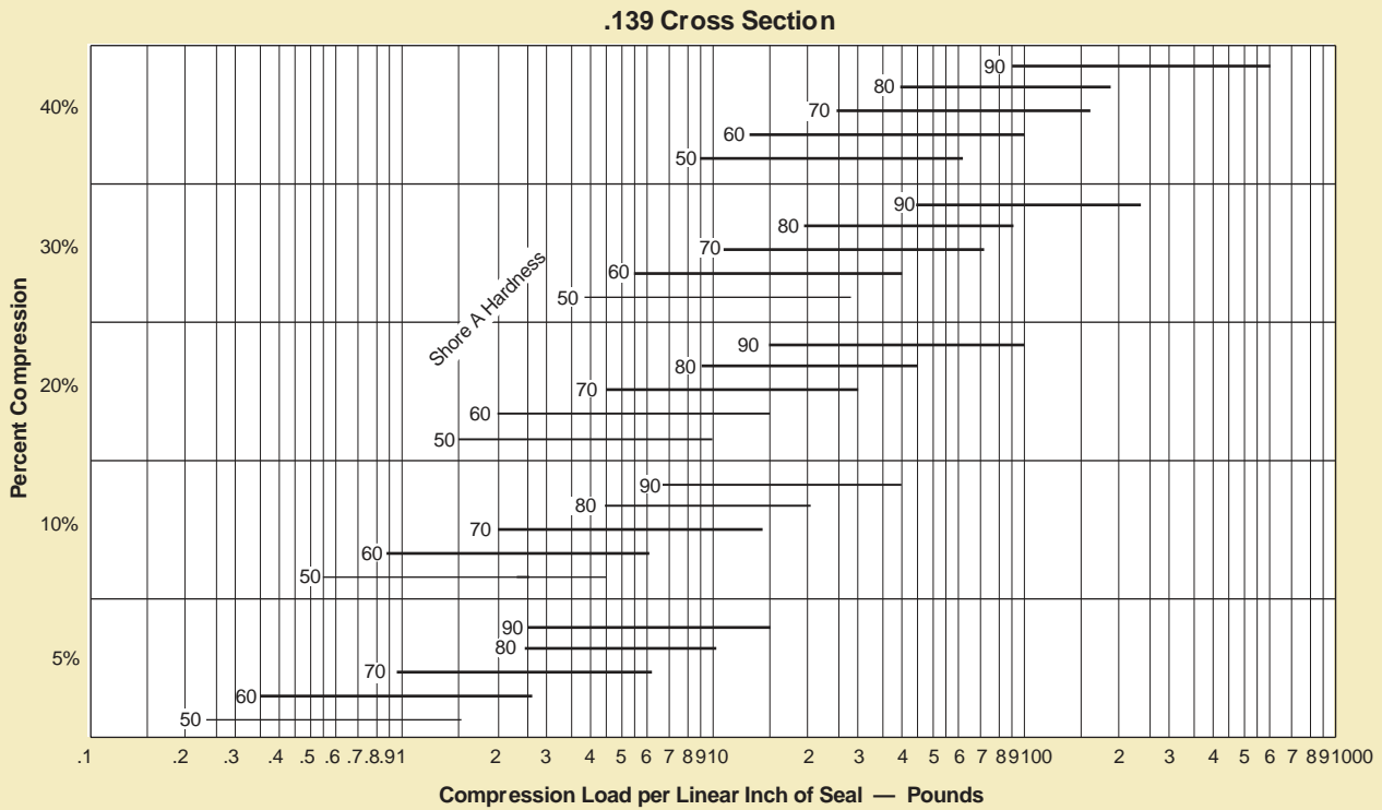
Figure 2-6: .139 Cross Section
