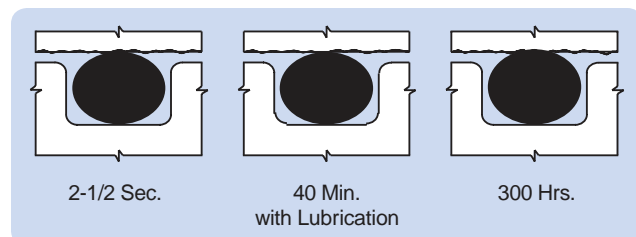
Figure 5-8: Flow of O-Ring into Metallic Surfaces
