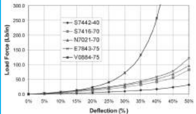
Chart 18 - Square (Edge = .066")
