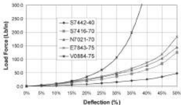
Chart 19 - Square (Edge = .099")
