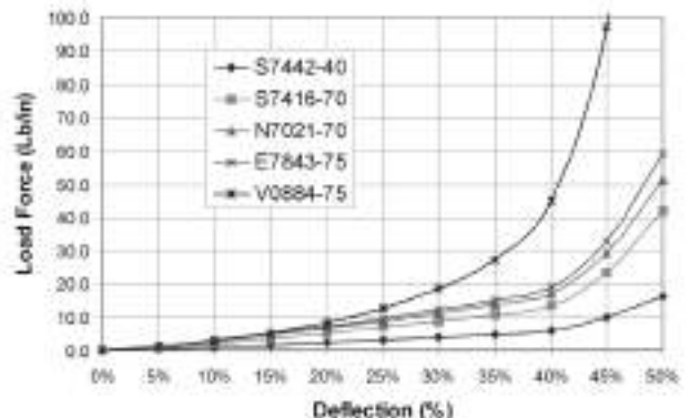
Chart 12 - Hollow-O (O.D. = .156", I.D. = .050")
