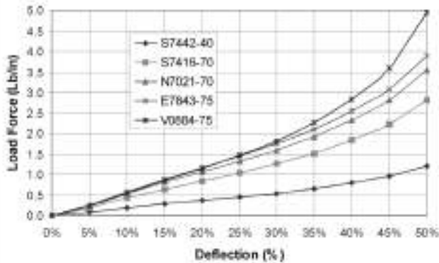
Chart 13 - Hollow-O (O.D. = .156", I.D. = .096")
