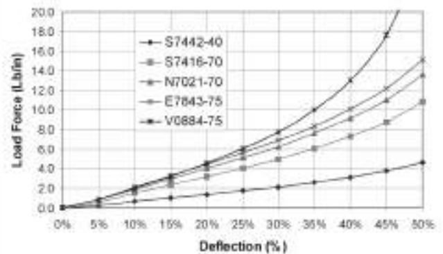
Chart 16 - Hollow-O (O.D. = .250", I.D. = .125")
