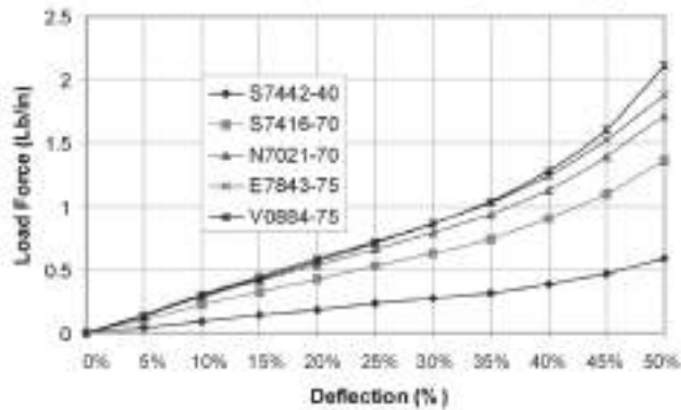
Chart 15 - Hollow-O (O.D. = .210", I.D. = .150")
