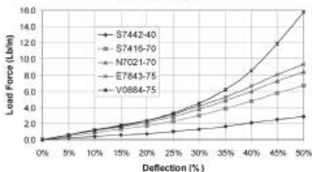
Chart 22 - Hollow-D (A = .312", B = .156", C = .156", D = .045")
