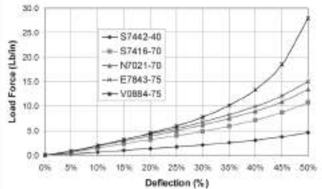
Chart 14 - Hollow-O (O.D. = .210", I.D. = .100")
