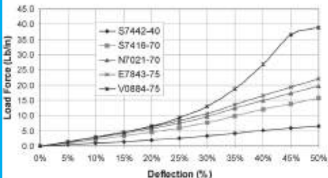
Chart 24 - Hollow-D (A = .312", B = .156", C = .156", D = .062")
