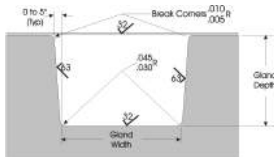
Figure 4 - Typical Gland Surface Finish
