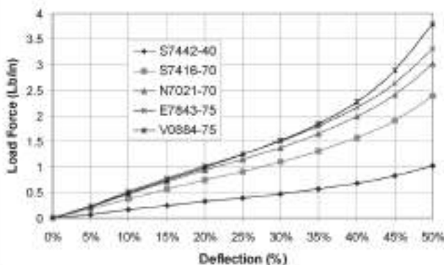
Chart 17 - Hollow-O (O.D. = .250", I.D. = .170")
