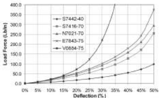
Chart 20 - Square (Edge = .203")
