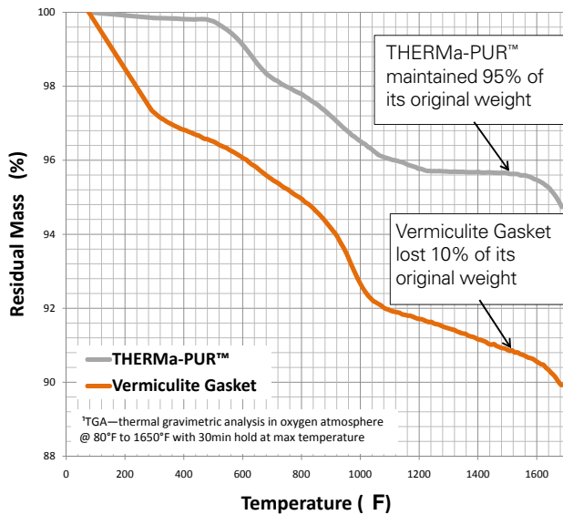
Weight Loss Testing (TGA¹)
